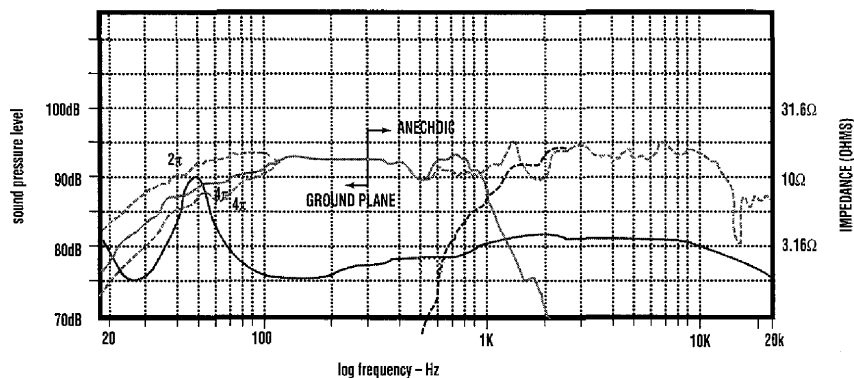
Figure 5. S2600 Frequency Response & Impedance
