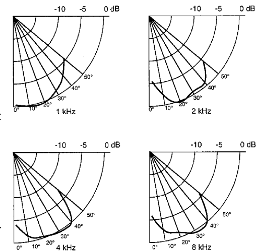
Figure 4. Horizontal polar response for the left channel loudspeaker.
