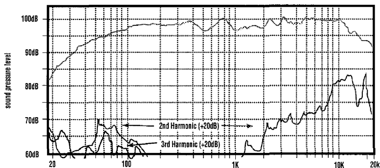
Figure 6. S2600 2nd & 3rd Harmonic Distortion
